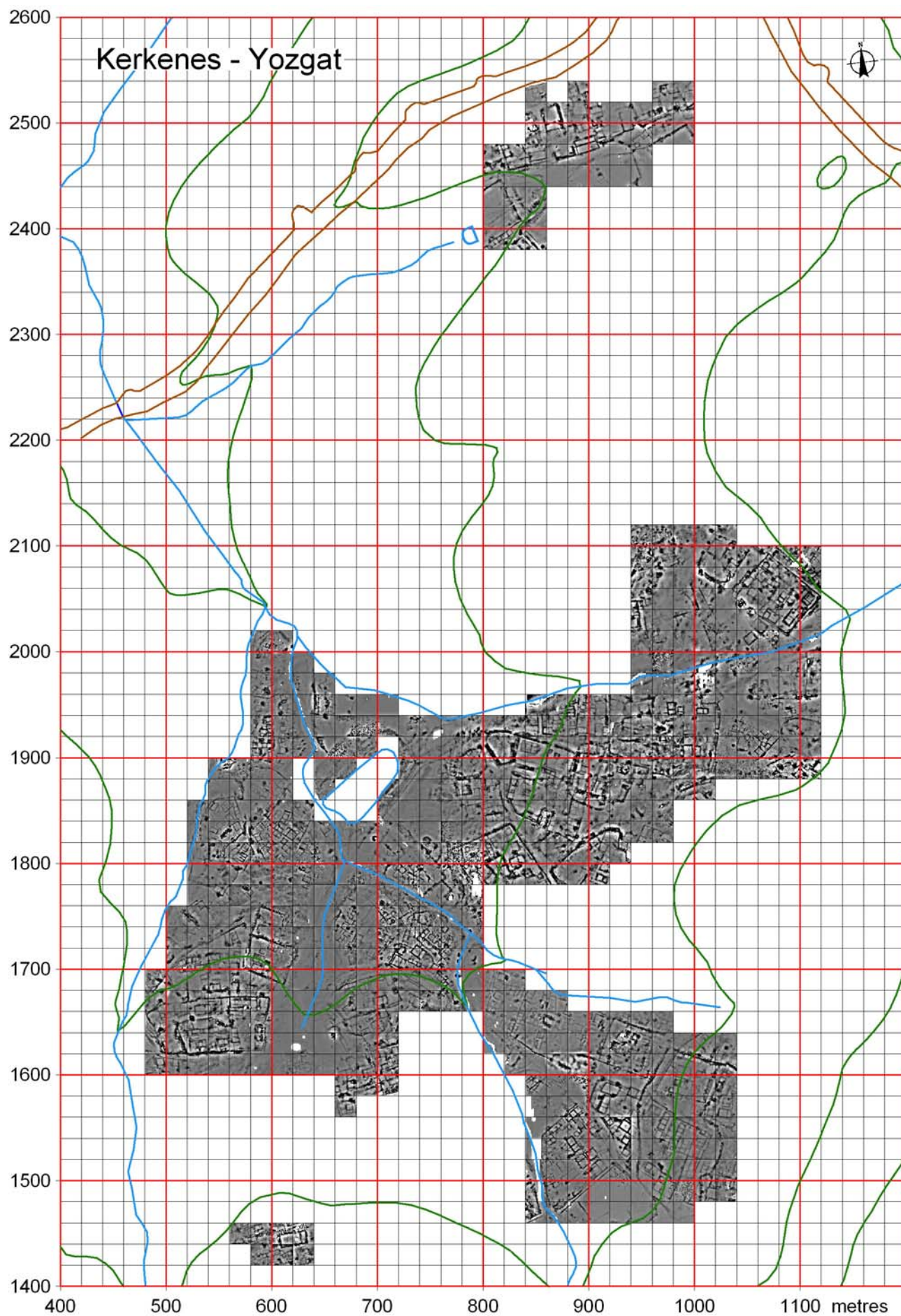
Figure 11. Area of resistivity conducted during the survey seasons of 2001 to 2005.
